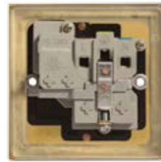
Angled in-line colour coded captive terminals
